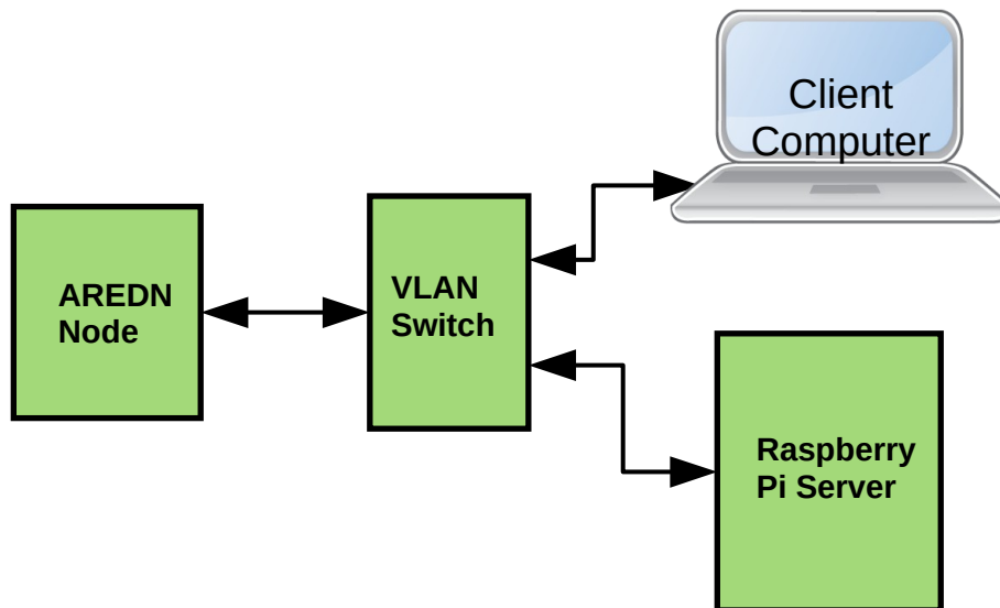
Figure 3. Raspberry Pi connected to VLAN switch provides services to the mesh network. Services may include web, file storage, chat, Winlink post office, and PBX.
